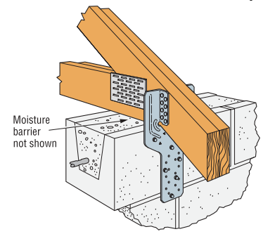
Typical LGT2 Installation into Concrete
