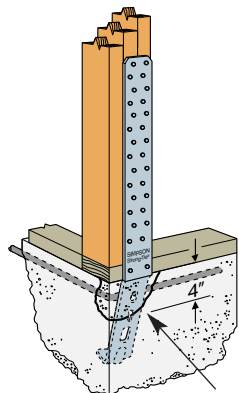
Typical STHD Edge Installation (for two pour, see footnote 5.)
