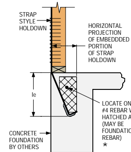
Single Pour Rebar Installation *Maintain minimum rebar cover, per ACI-318 concrete code requirements.
