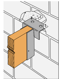
Typical WM Installation
