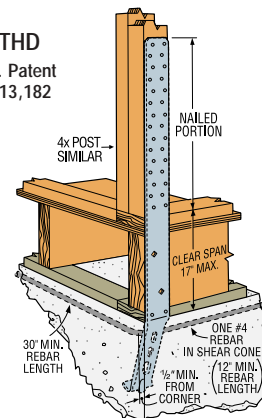
Typical STHD14RJ Rim Joist Application
